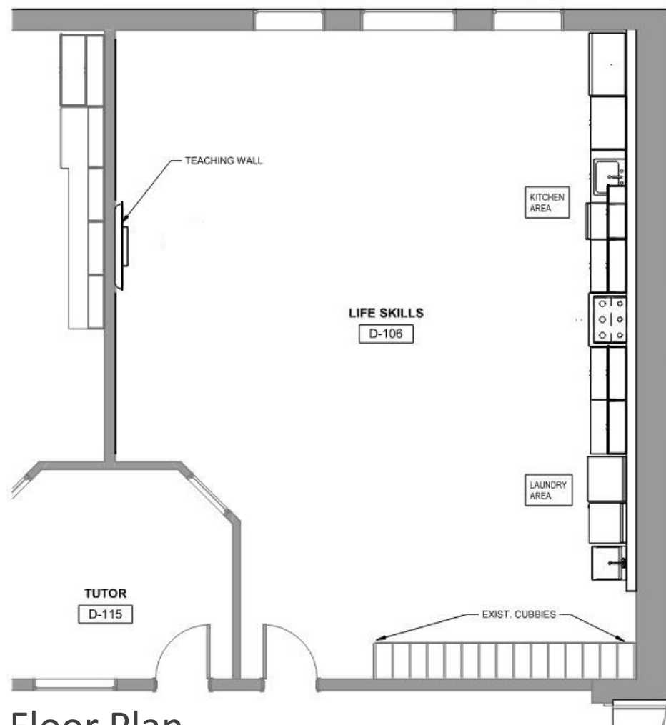
Floor Plan
